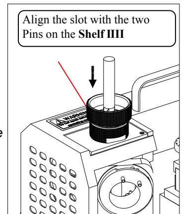
Diagram:4-10 Shelf IIII
