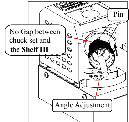
Diagram:4-9 Shelf III
